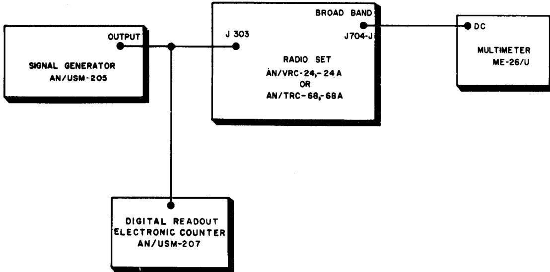
Figure 117. Bandwidth/selectivity test.
