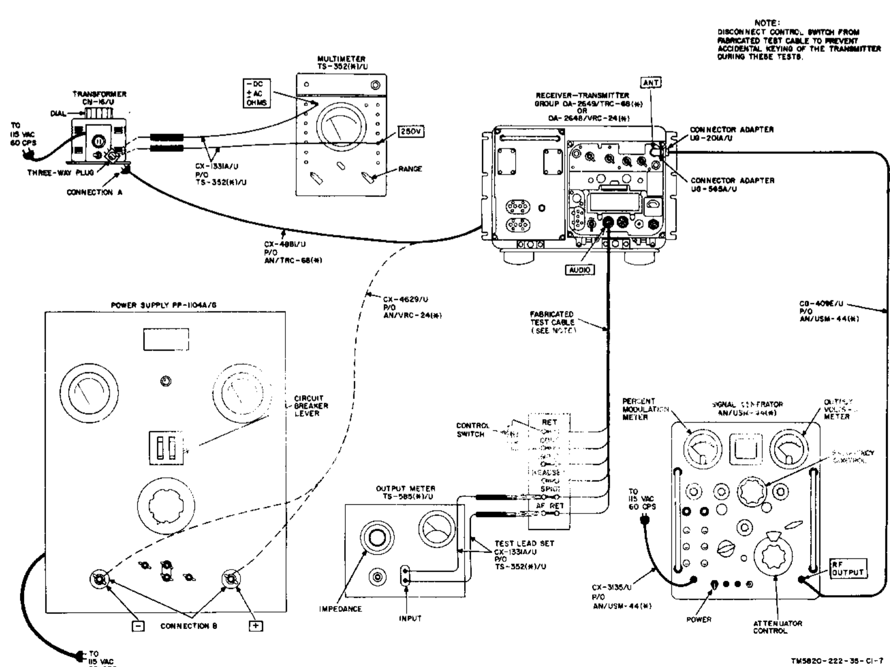
Figure 115.7. RT-393/VRC-24(*) or RT-441/TRC-68(*) receiver sensitivity, resetability, audio output, signal plus noise-to-noise, and squelch tests, test setup.
