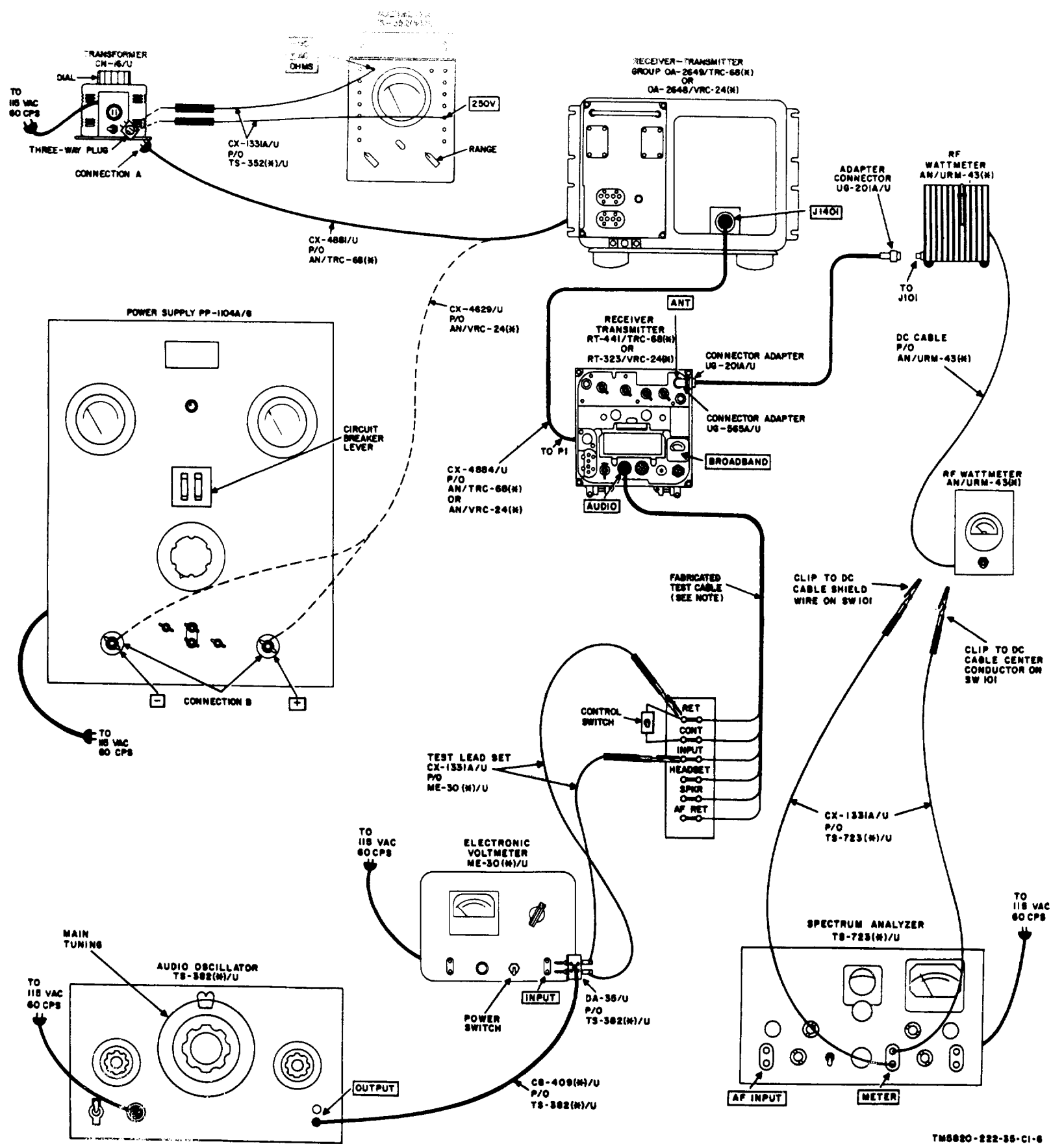
Figure 113.6 RT-323/VRC-24 or RT-441/TRC-66 transmit frequency response, carrier noise, and distortion tests, test setup.
